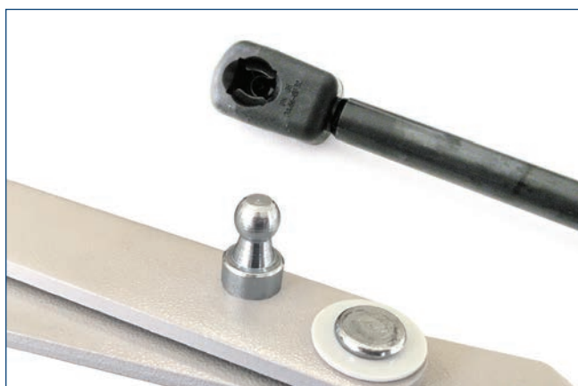
Attacco rapido / Ball-joint end fitting
